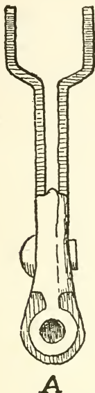
A Spread Check Fork May Cause Stringing
